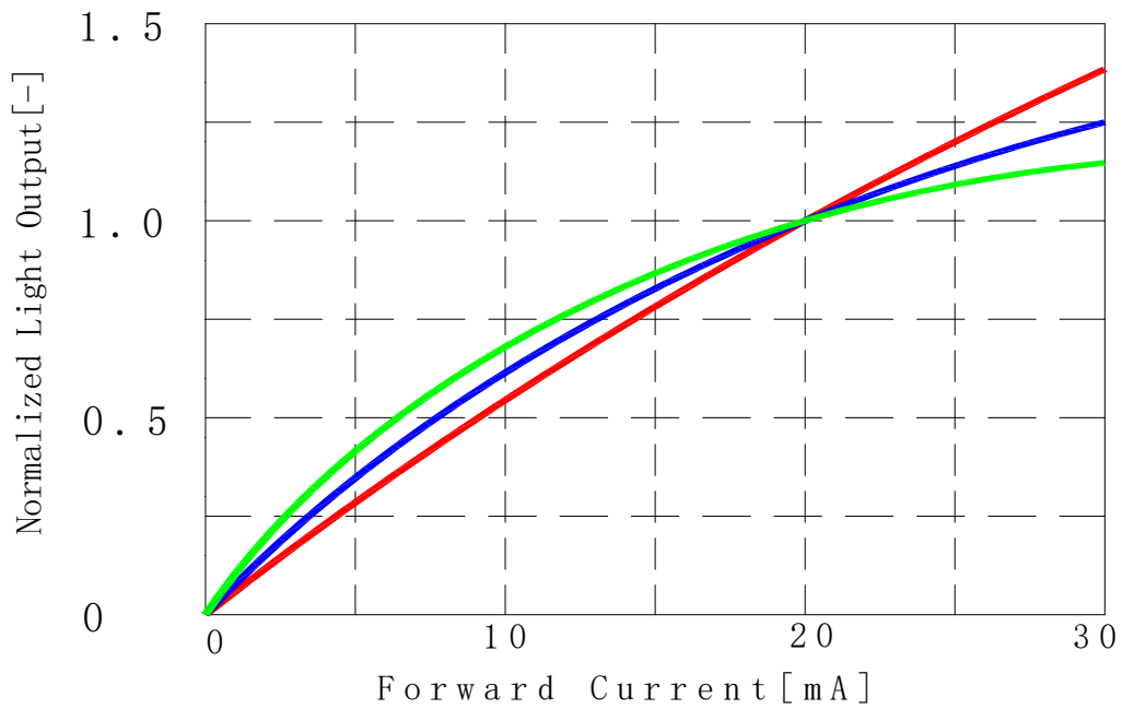
Figure 3. Typical normalized light output vs. forward current for Lumileds 5050 RGB R at T=25^{\circ}\text{C}
