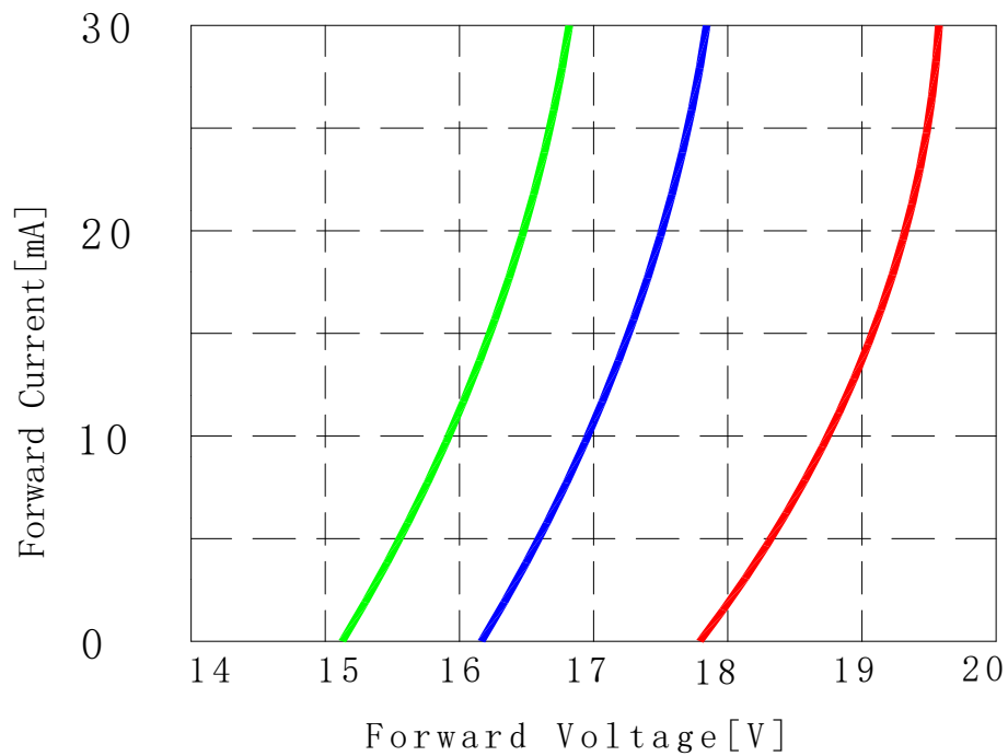
Figure 4. Typical forward current vs. forward voltage for Lumileds 5050 RGB R at T=25^{\circ}\text{C} .
