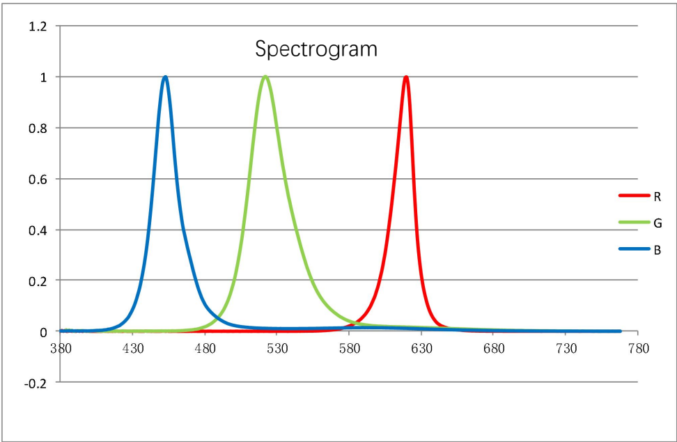
Figure1 . Typical normalized power vs. wavelength for Lumileds 5050 RGB R at 20mA, T=25 °C
