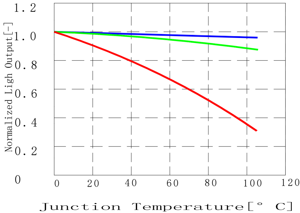
Figure 2 . Typical normalized light output vs . junction temperature for Lumileds 5050 RGB R at 20mA .
