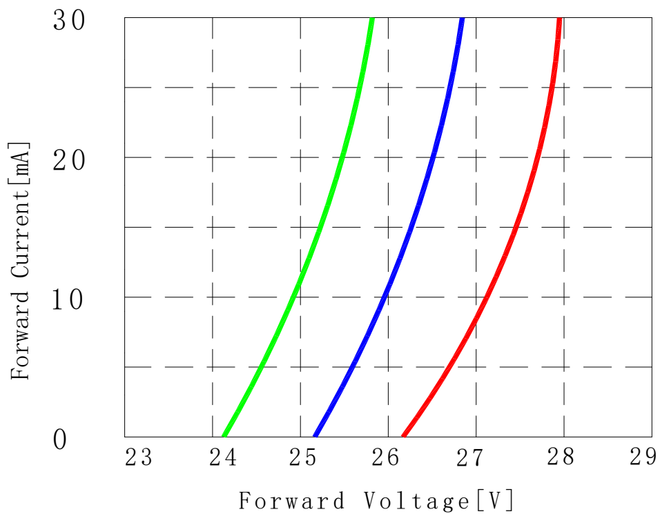
Figure 4. Typical forward current vs. forward voltage for Lumileds 5050 RGB R at T=25°C.
