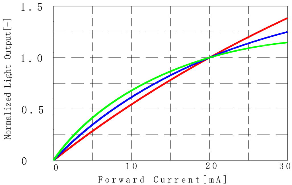
Figure 3. Typical normalized light output vs. forward current for Lumileds 5050 RGB R at T=25°C
