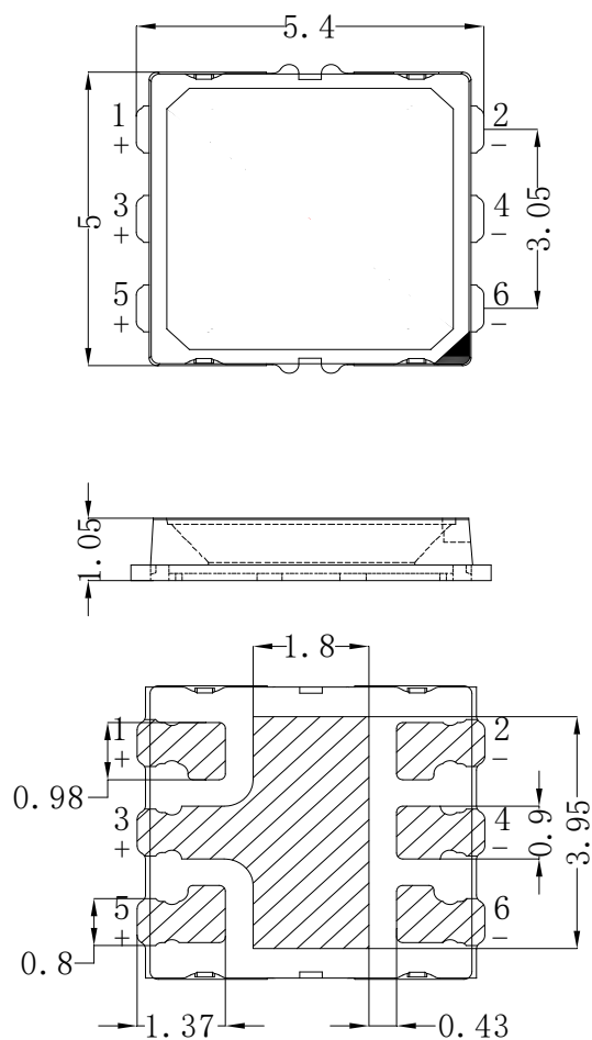
Figure. Mechanical dimension
