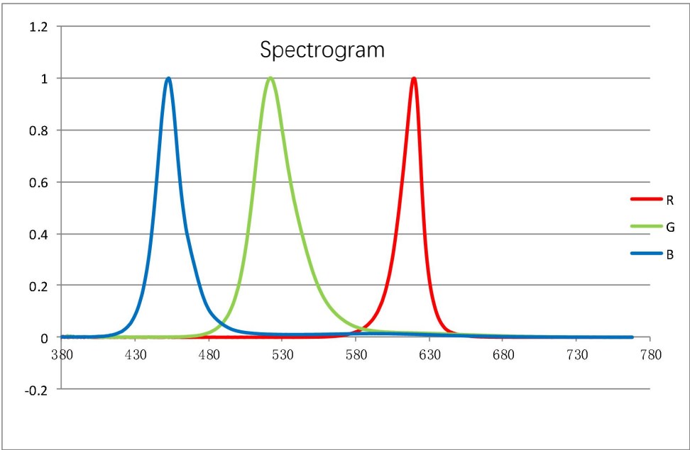
Figure1 . Typical normalized power vs. wavelength for Lumileds 5050 RGB R at 30mA, T=25 °C
