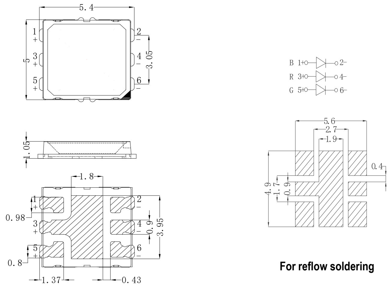
Figure. Mechanical dimension
