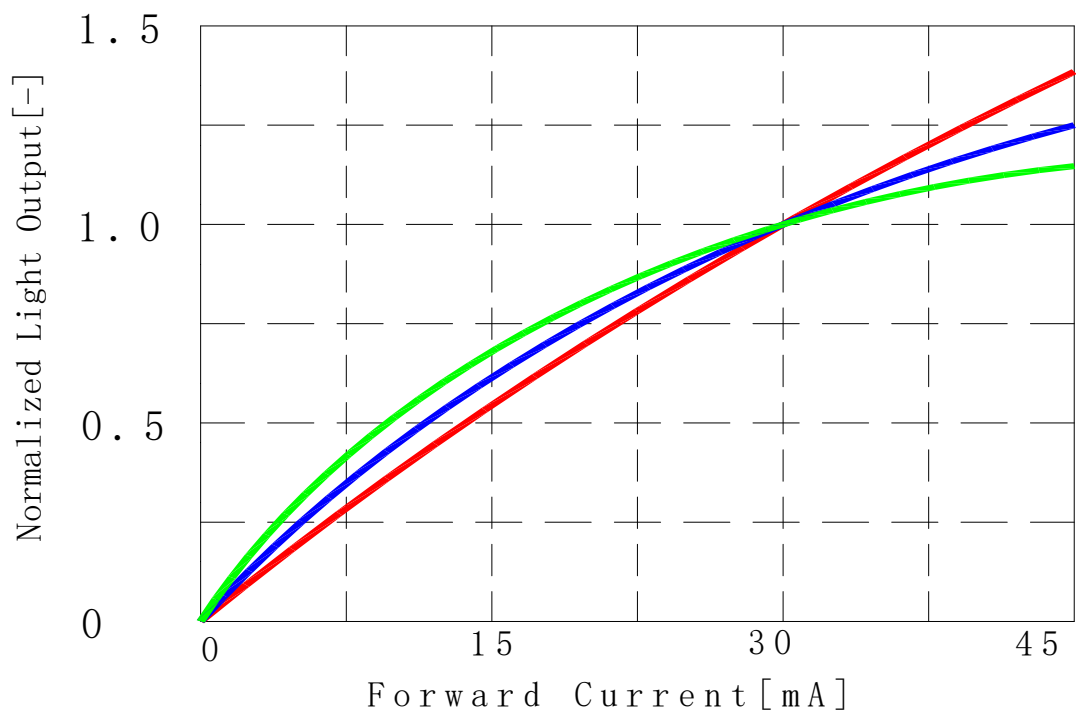
Figure 3. Typical normalized light output vs. forward current for Lumileds 5050 RGB R at T=25^{\circ}\text{C}
