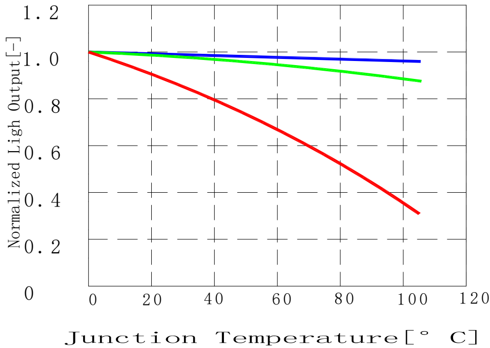
Figure 2 . Typical normalized light output vs . junction temperature for Lumileds 5050 RGB R at 30mA .
