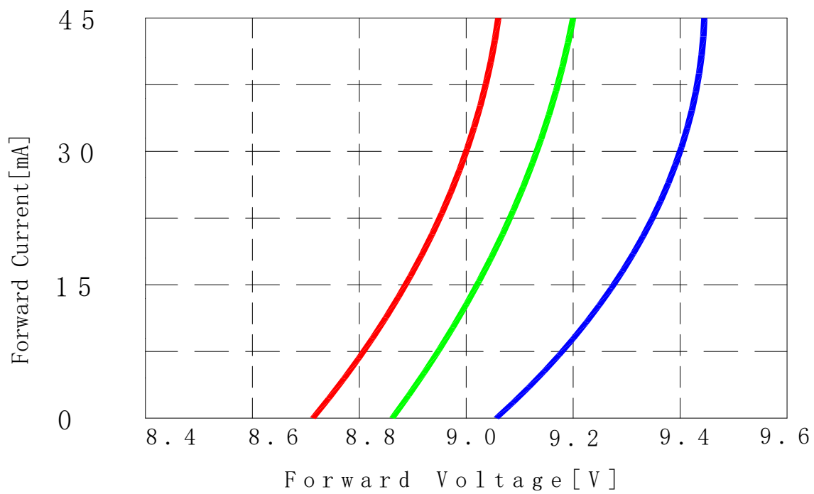
Figure 4. Typical forward current vs. forward voltage for Lumileds 5050 RGB R at T=25^{\circ}\text{C} .
