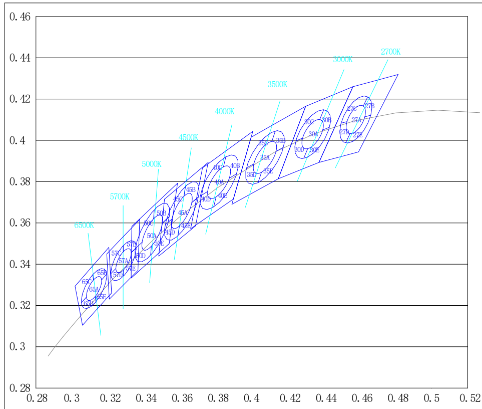
Correlated color temperature bin definitions for 2835R Series at rated current, Ta=25°C
